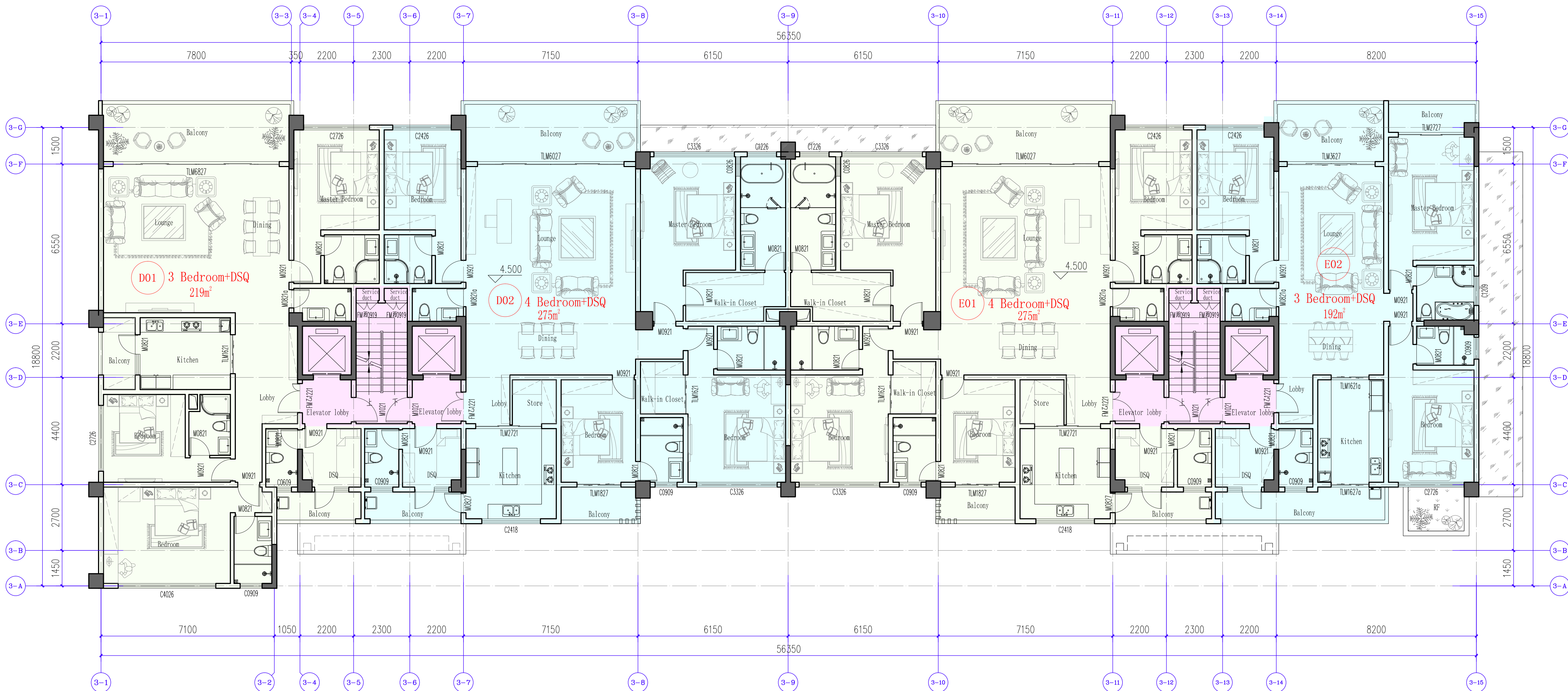
3# 1 FLOOR PLAN (BLOCK D, E)
