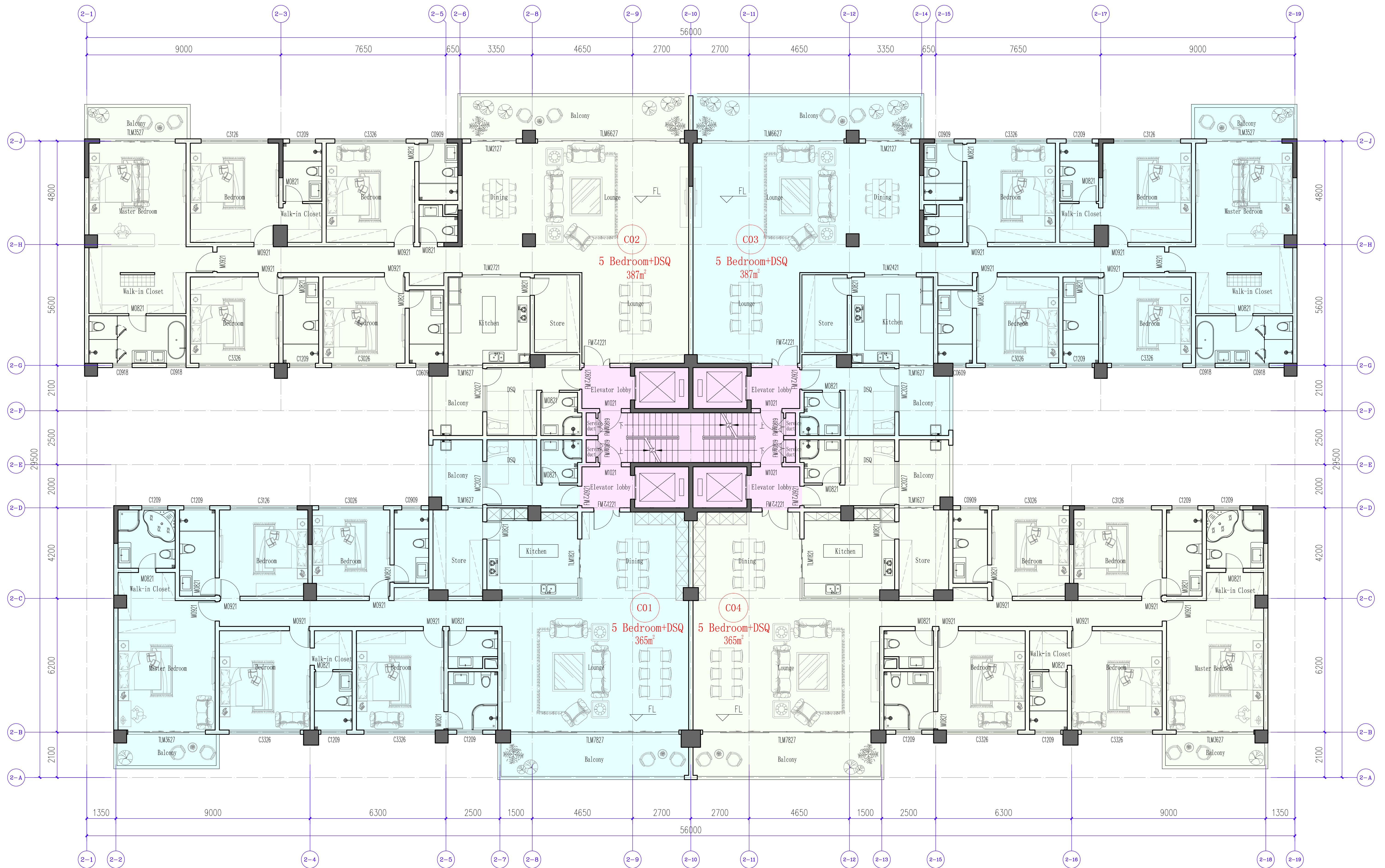
2# TYPICAL FLOOR LAYOUT PLAN (BLOCK C)
